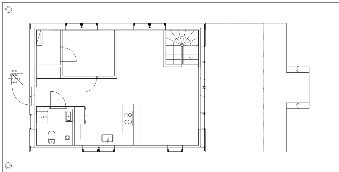
Plan 1, Entreplan 52m 2
