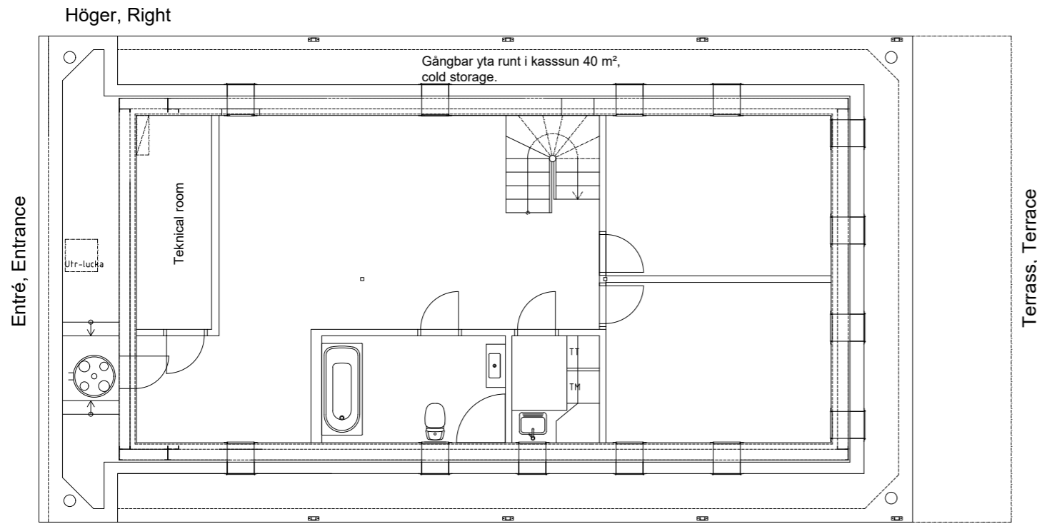
Plan 0, Kassunplan 78m 2
