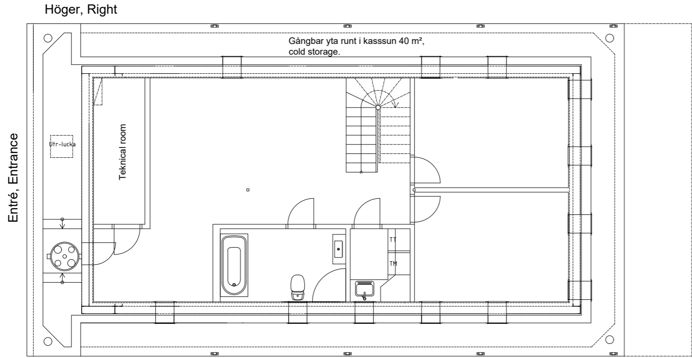
Plan 0, Kassunplan 78m 2
